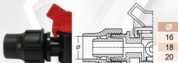
Quick Coupling (Lock) Ρακόρ (Lock)
