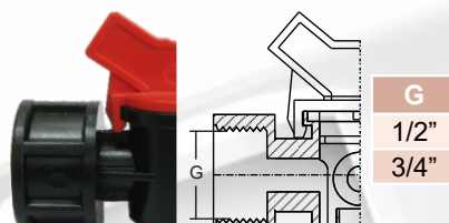
Nipple Female threaded Νίπελ Θηλυκό
